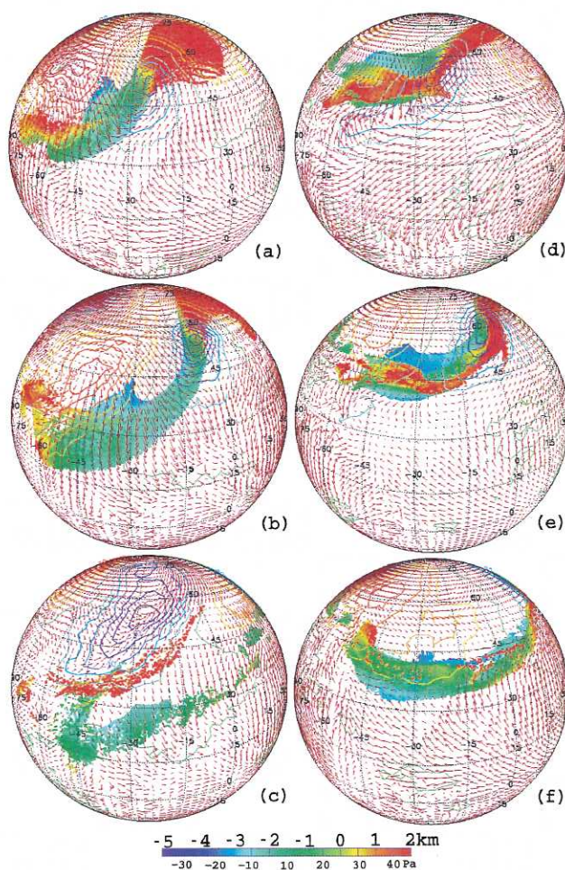
Figure 2. Lagrangian particle evolution for a front (a–c) with significant southward motion at Ls 342° and (d–f) without significant southward motion at Ls 354. The projection is that used in Figure 1. The altitudes of the particles are color-coded above the color bar. High particles are plotted above low ones. Simultaneous ~130 m model winds and surface pressure perturbation (contours, color-coding below the color bar) are shown. The particles are advected for 16 hr in (a, d), 48 hr in (c, f), 24 hr in (b) and 28 hr in (e). Low pressure centers pass 0°E in (b, e). The local time at -35°E is (b) 11:40 am and (e) 3:40 am.
