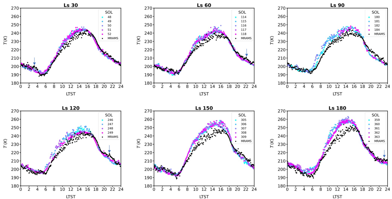
Figure 3. MEDA air temperature at \sim 1.45 m measured by the ATS1 within five sols of the given L_s (colored dots) and Mars Regional Atmospheric Modeling System (MRAMS) data taken from the lowest model level at \sim 14.5 m (black dots). Blue arrows represent examples of times when the model predicts thermal perturbations at the same times as the increases of TKE shown in Figure 6.
