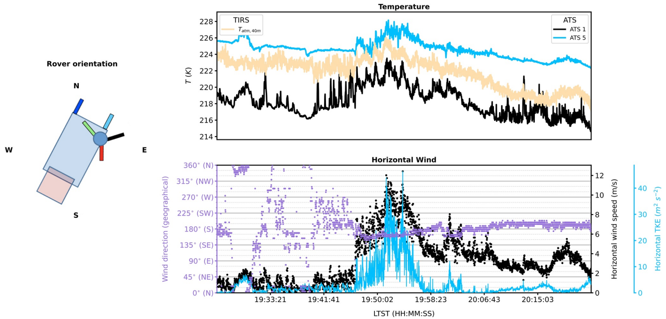
Figure 2. (left) The rover orientation for this period and placement of the five Air Temperature Sensors (ATS1 and ATS5 colorized as in the upper right-hand plot), to aid in analyzing thermal contamination from the rover's RTG and deck. (right) MEDA data from 19:25 through 20:25 on sol 213 ( L_s 104), showing (top) 0.85 m ATS5 air temperatures (light blue line), 1.45 m ATS1 air temperatures (black line), and ~40 m air temperature (cream line), and (bottom) wind direction (purple dots), wind speed (black dots) and TKE_H (light blue line, derived from MEDA wind speeds as shown in the text) fluctuations.
