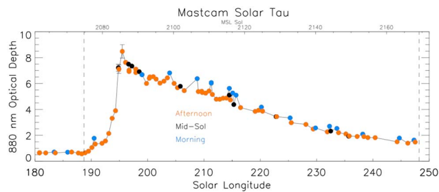
Figure 1. Mastcam 880-nm atmospheric optical depth during the 2018/MY34 global dust storm plotted against solar longitude and Mars Science Laboratory (MSL) mission sol number. One-sigma error bars are plotted for all points (but only visible for a few points). Points are color coded based on local true solar time (LTST) of observation with “Morning” defined as 0700–1000 LTST, “Mid-Sol” as 1000–1400 LTST, and “Afternoon” as after 1400 LTST. Dashed-vertical lines indicate when the MSL global dust storm campaign started and stopped.
